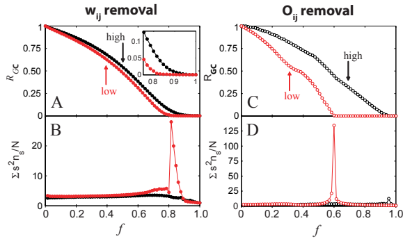
Figure 3. Robustness of the communication network with respect to edge removal. (A, B) Edges are removed on the basis of their weights. The black curves correspond to removing strong edges first, while the red curves denote the opposite, starting from weakest edges. (A) shows the relative size of the largest component as a function of fraction of removed edges; removing weak links first fragments the network at around f = 0.8 (see also inset). This is corroborated by the susceptibility peak in panel (B). (C,D) For reference, edges are removed in order of their overlap O_{ij} and the panels again display the relative largest component size and susceptibility. Removing low-overlap edges first rapidly breaks the network apart, reflecting the weight-overlap dependence shown in Fig. 2.
